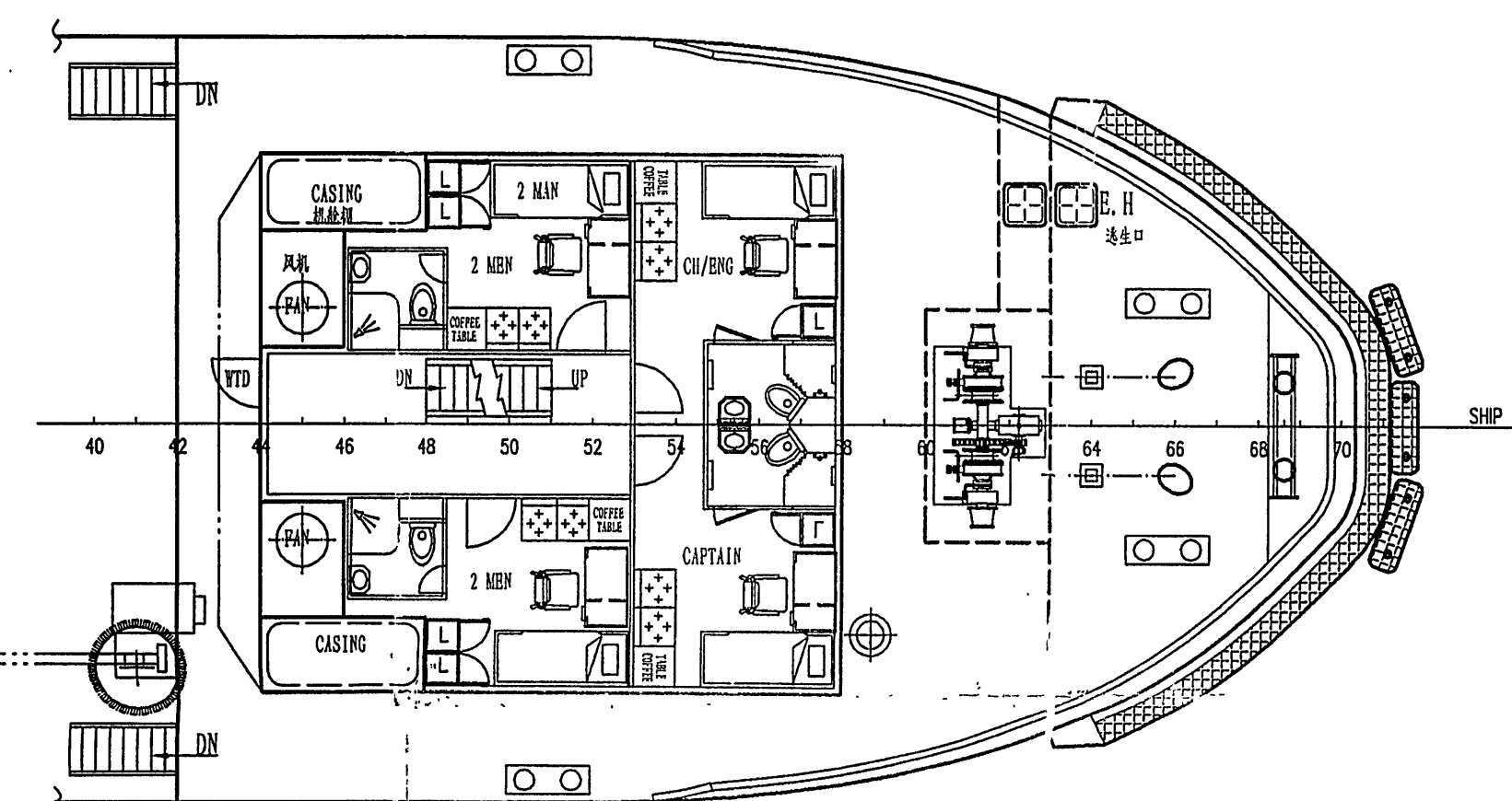
FORECASTLE DECK
