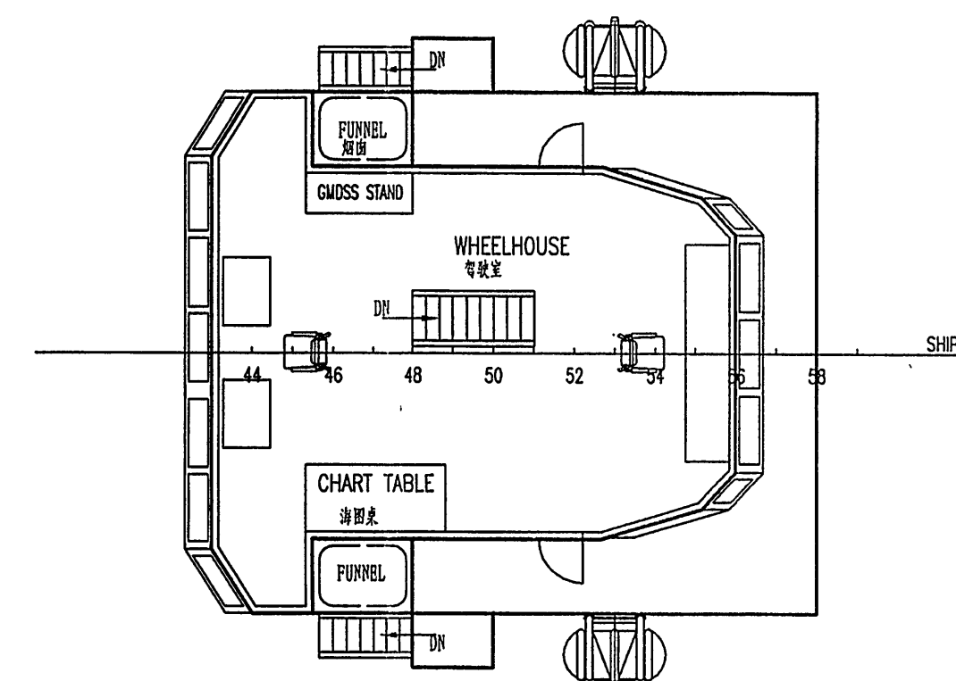
WHEELHOUSE DECK PLAN
